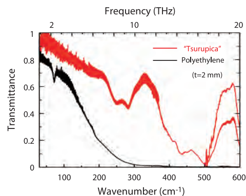
Tsurupica transmittance in THz region
